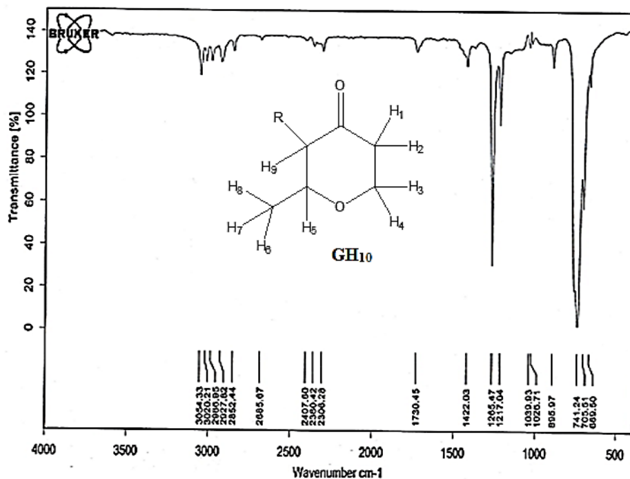
Figure 7. FT-IR spectrum of compound GH10
