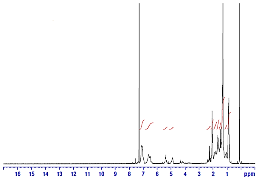
Figure 14. 1 H NMR Spectrum of compound 2C8
