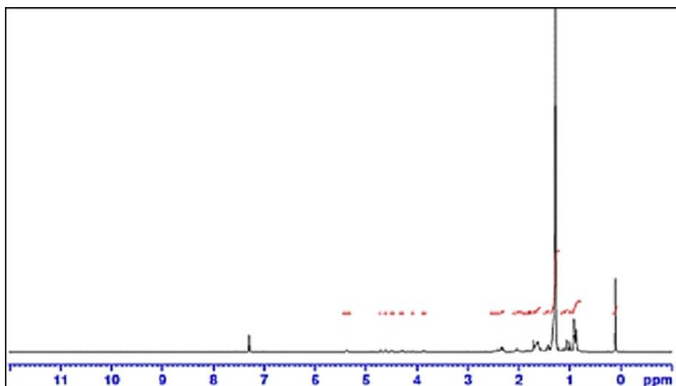
Figure 8. ^1\text{H} NMR spectrum of compound GH10
