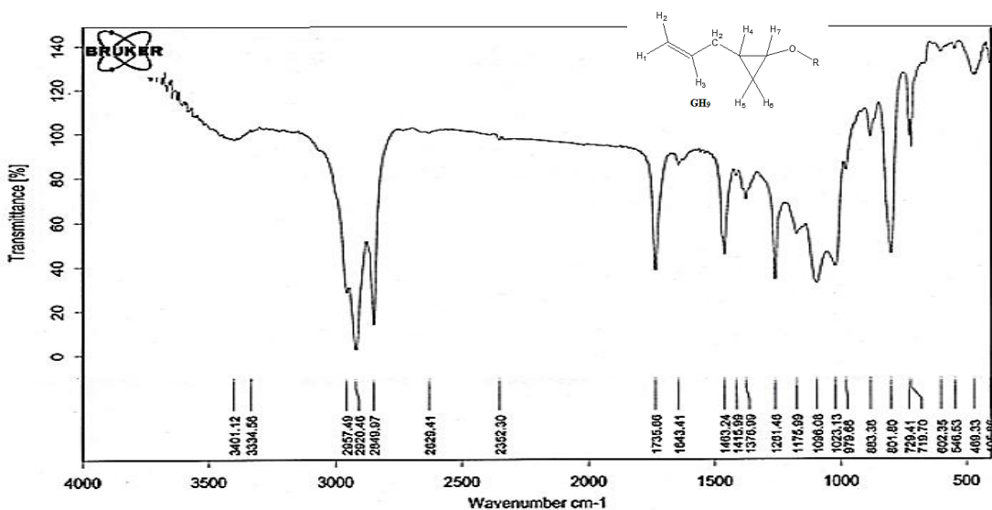
Figure 5. FT-IR spectrum of compound GH9
