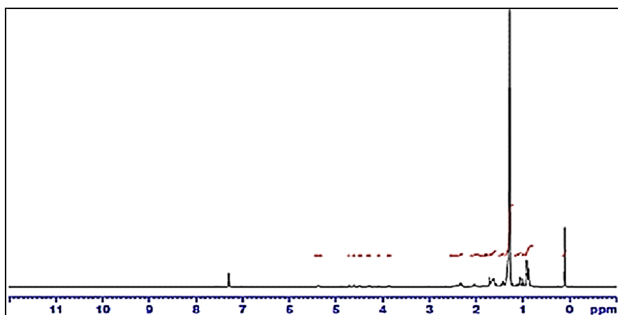
Figure 6. 1 H NMR spectrum of compound GH9
