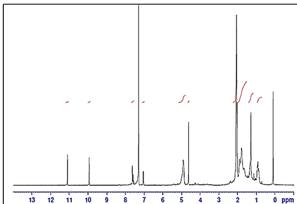
Figure 4. 1 H NMR spectrum of compound 2C7
