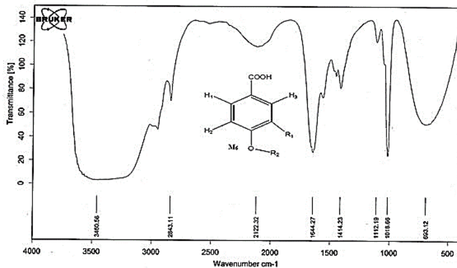
Figure 9. FT-IR spectrum of compound M6
