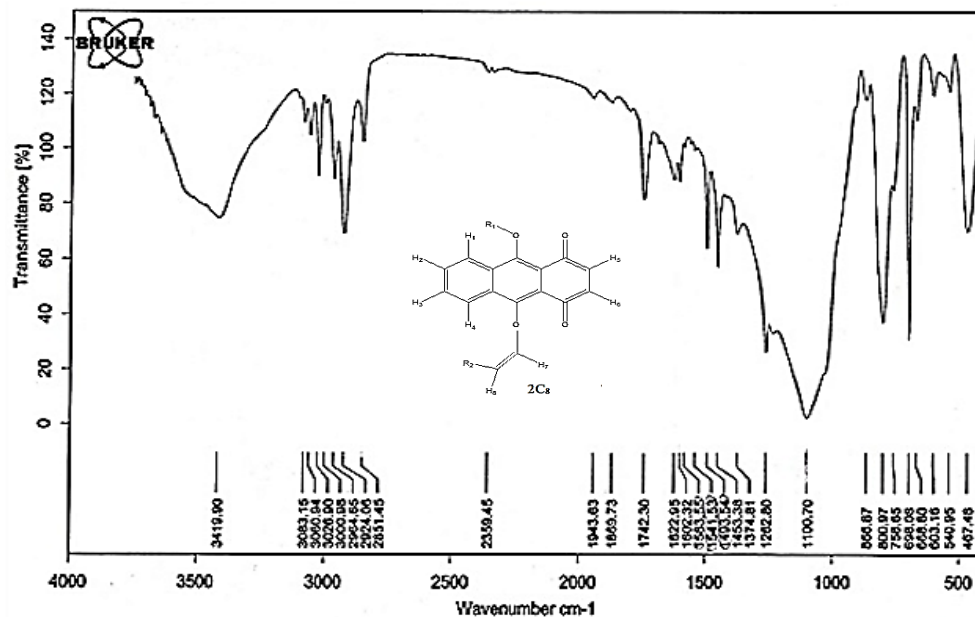
Figure 13. FT-IR Spectrum of compound 2C8
