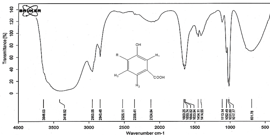
Figure 3. FT-IR spectrum of compound 2C7
